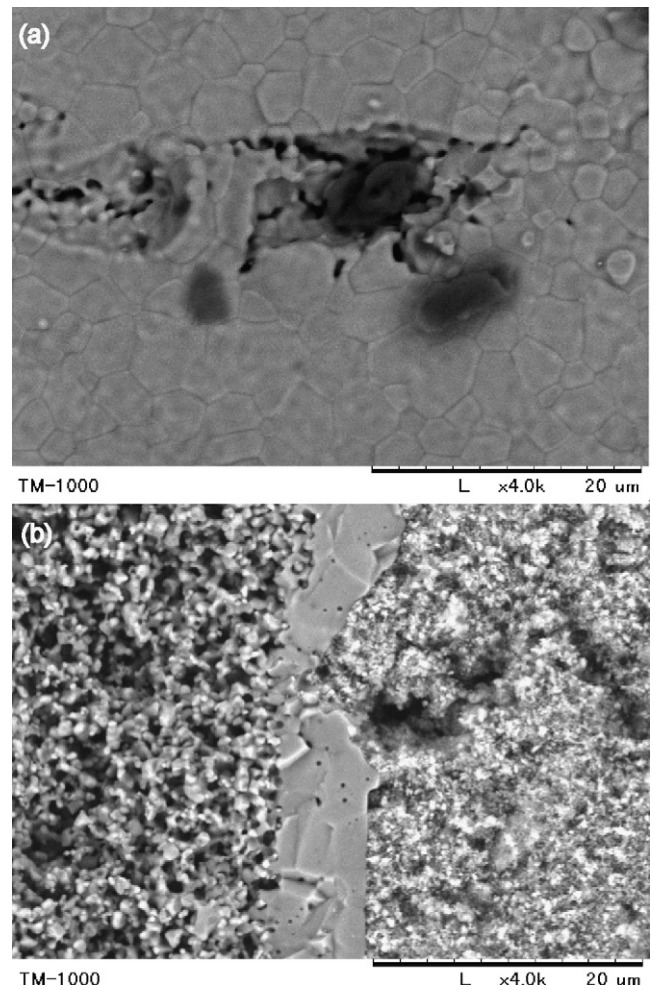
Fig. 4. (a) Micro-cracks on free electrolyte surface. (b) Micro-cracks at anode-electrolyte-cathode cross-section.
